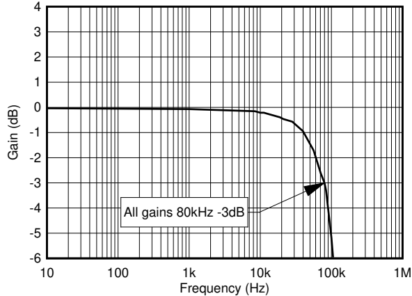
Figure 6-9. Sensitivity vs Frequency, All Gains Normalized to 1Hz
