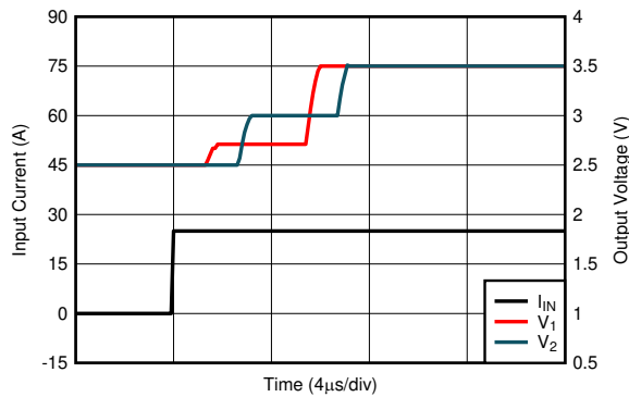
Figure 6-17. Voltage Output Step, Rising
