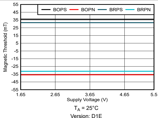
Figure 6-8. 30mT Magnetic Threshold vs Supply
