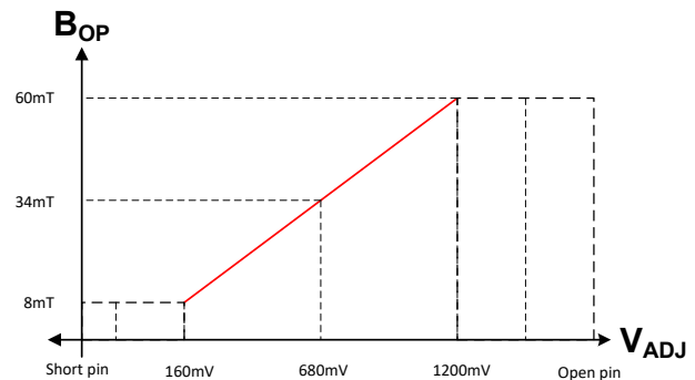
Figure 7-8. B_{OP} vs V_{ADJ} (D1E version)
