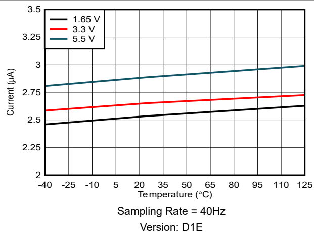
Figure 6-12. Average I_{CC} vs Temperature
