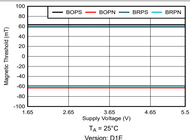
Figure 6-10. 60mT Magnetic Threshold vs Supply
