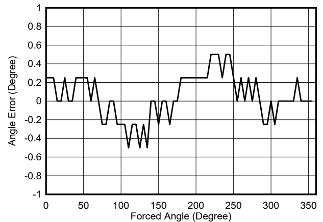
Figure 6-20. Angle Error at 25°C, X-Z Configuration, 50-mT Range
