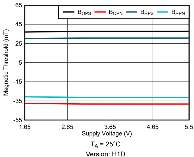
Figure 6-10. 37mT B_{OP} : Thresholds vs Supply Voltage
