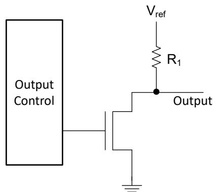
Figure 7-8. Open-Drain Output (Simplified)
