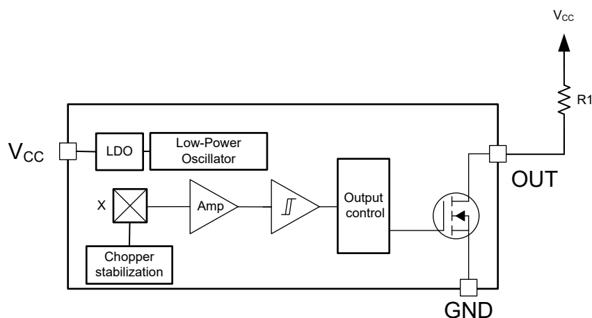
Figure 7-2. Block Diagram (Open-Drain)
