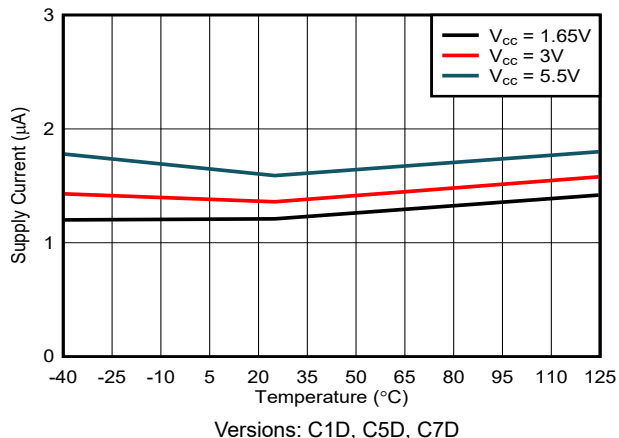
Figure 6-12. 20Hz: Average I_{CC} vs Temperature
