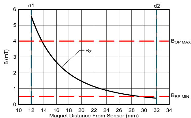
Figure 8-9. B-Field Hypothesis Two
