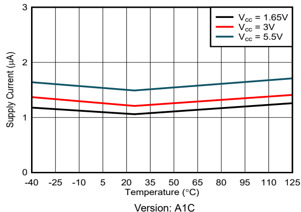
Figure 6-11. 10Hz: Average I_{CC} vs Temperature
