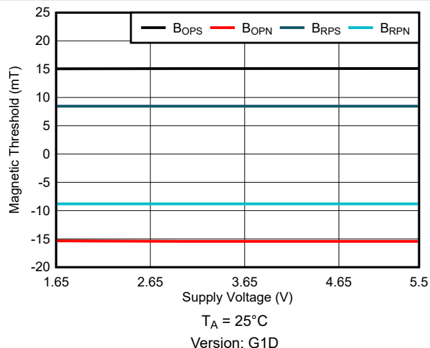
Figure 6-8. 15mT B_{OP} : Thresholds vs Supply Voltage
