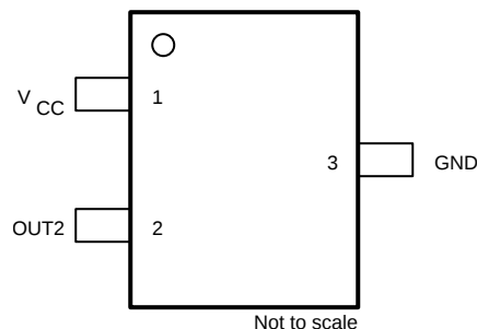
Figure 5-2. DBZ Package 3-Pin SOT-23 (Top View): C5D Version
