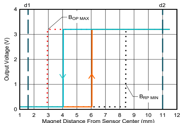
Figure 8-13. Thresholds From Hypothesis One
