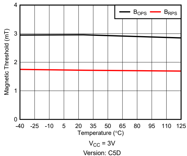
Figure 6-5. 3mT B_{OP} , 1.2mT B_{HYS} : Thresholds vs Temperature
