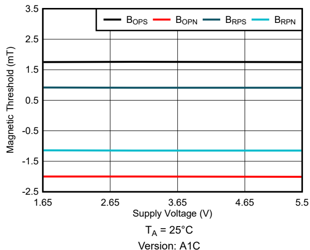
Figure 6-2. 1.8mT B OP : Thresholds vs Supply Voltage
