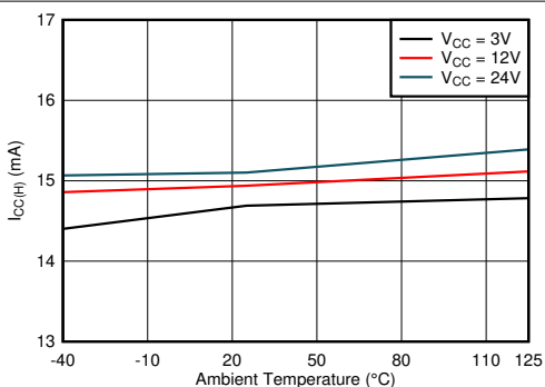
Figure 7-29. I_{CC(H)} vs. Temperature
