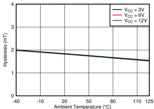
Figure 7-11. Hysteresis vs Temperature
