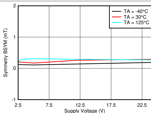
Figure 6-23. B_{SYM(Y)} vs V_{CC}
