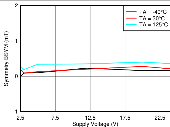
Figure 6-19. B_{SYM(Z)} vs V_{CC}
