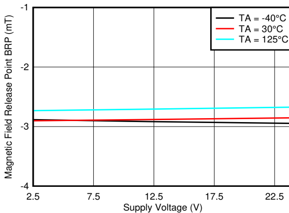
Figure 6-41. B_{RP\_Z} Threshold vs V_{CC}
