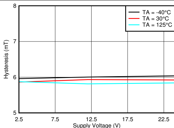
Figure 7-43. Hysteresis_Z vs. V CC
