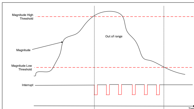
Figure 8-6. Magnitude Limit Cross Check With MAG_THR_DIR = 0h, THR_SEL[1:0] = 3h, INT_State = 1h
