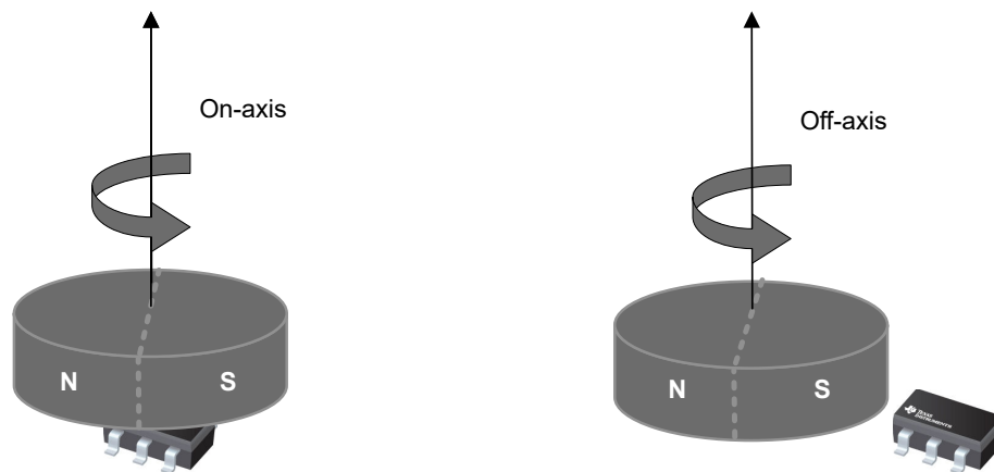
Figure 8-19. On-Axis vs Off-Axis Angle Measurements
