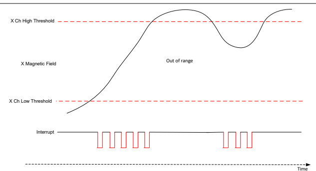
Figure 8-5. Magnetic Lower Limit Cross Check With MAG_THR_DIR = 1b, THR_SEL = 10b , INT_STATE = 1b
