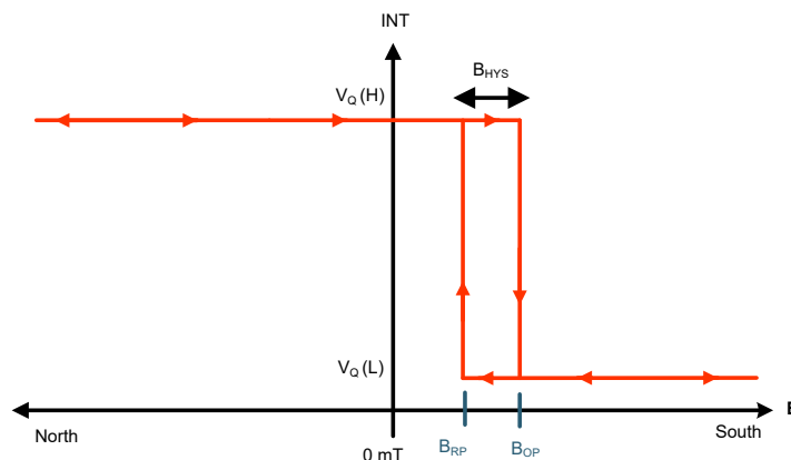
Figure 8-10. Unipolar 3D Magnetic Switch
