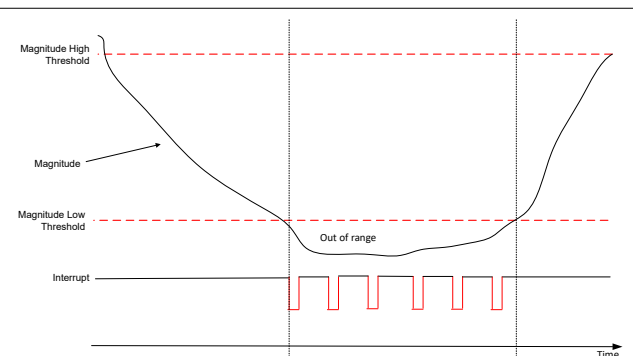
Figure 8-7. Magnitude Limit Cross Check With MAG_THR_DIR = 1h, THR_SEL[1:0] = 3h, INT_State = 1h
