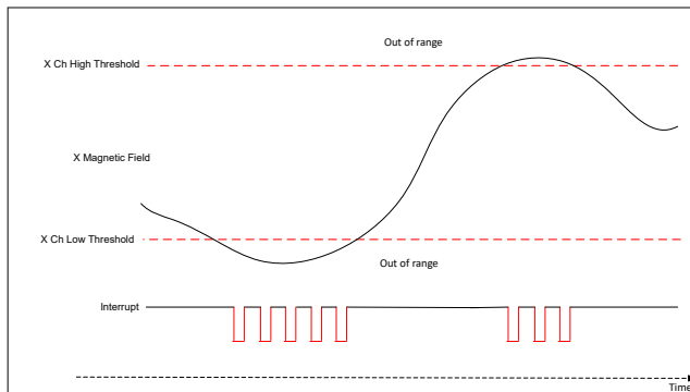
Figure 8-4. Magnetic Limit Cross Check With MAG_THR_DIR = 0h, THR_SEL[1:0] = 2h, INT_STATE = 1h
