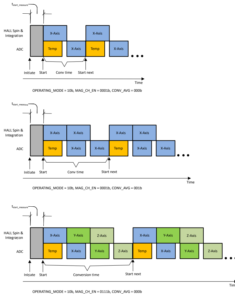
Figure 8-1. Continuous Conversion Examples
