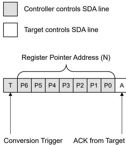
Figure 6-13. Control Register
