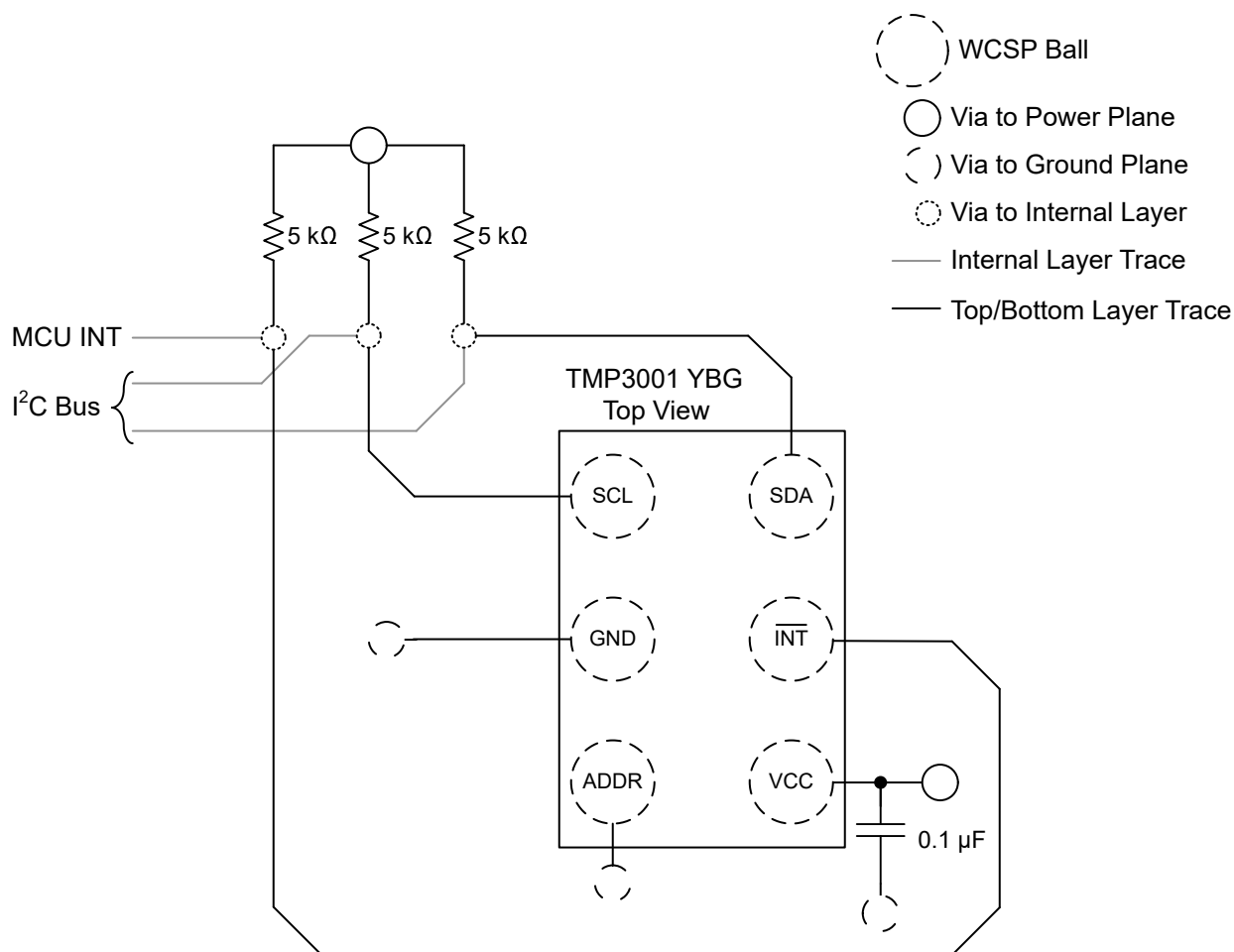
Figure 8-22. Layout Example With TMAG3001
