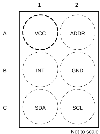
Figure 4-1. YBG (6 - DSBGA) Top View
