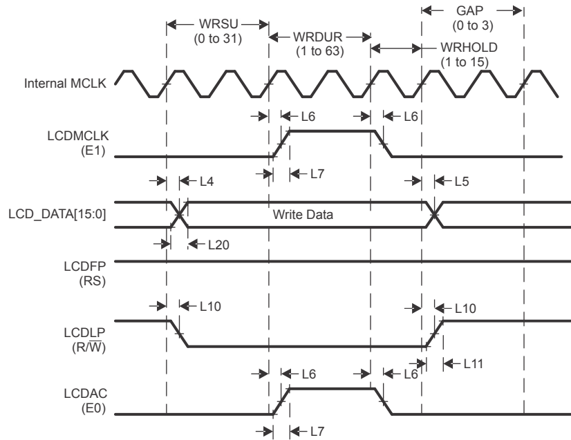
Figure 31-43. Data Write in Hitachi Mode
