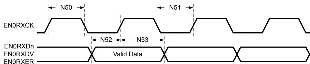
Figure 27-41. 10 Mb/s MII Receive Timing
