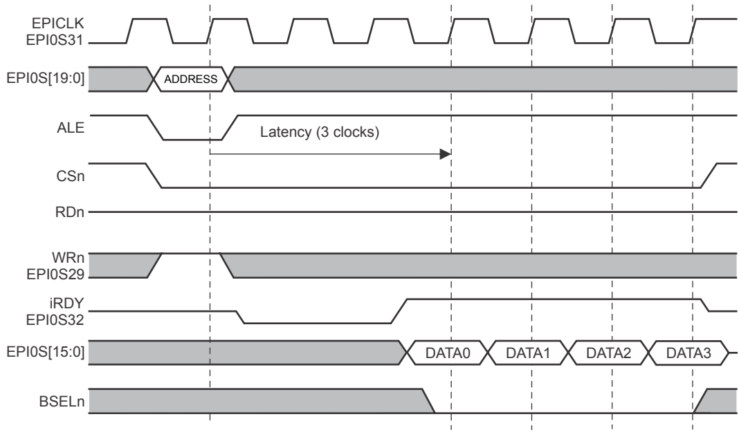
Figure 11-7. PSRAM Burst Read
