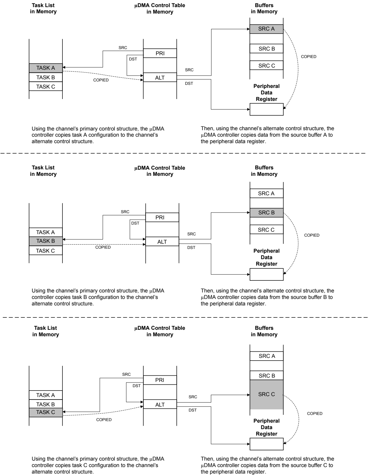
Figure 9-6. Peripheral Scatter-Gather, μDMA Copy Sequence
