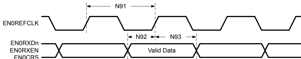
Figure 27-43. RMII Receive Timing
