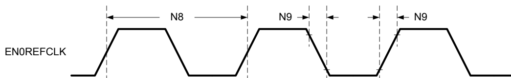
Figure 27-36. EN0RREF_CLK 50-MHz Oscillator Characteristics
