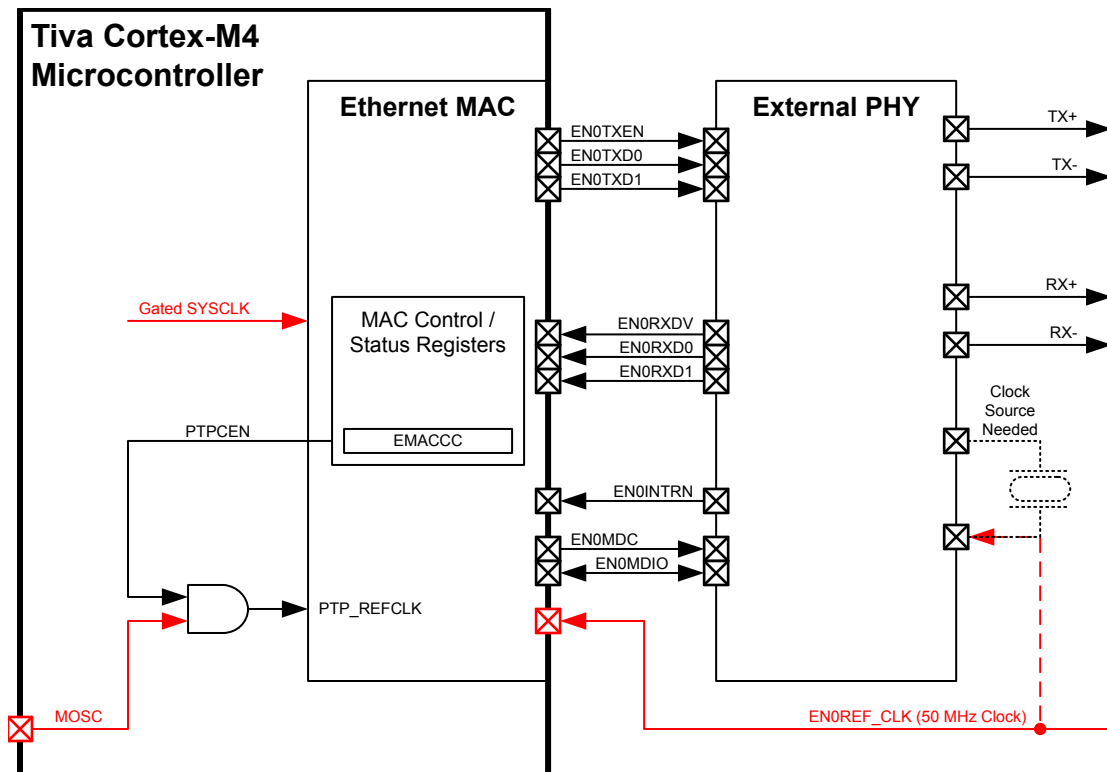
Figure 20-3. RMII Clock Structure
