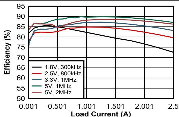
Figure 8-7. 24VIN Efficiency (Linear)
