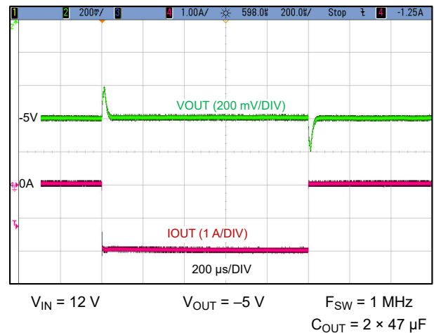
Figure 8-16. Load Transient 0 A to -2 A, 1 A/μs
