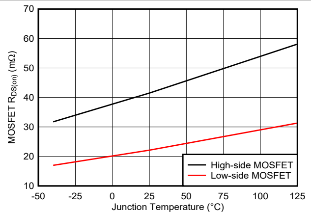
Figure 6-4. High-Side and Low-Side MOSFET R_{DS(on)}
