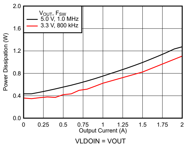
Figure 7-17. Power Dissipation
