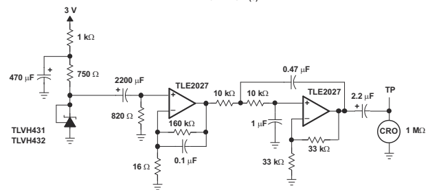
Figure 5-10. Equivalent Input Noise Voltage
