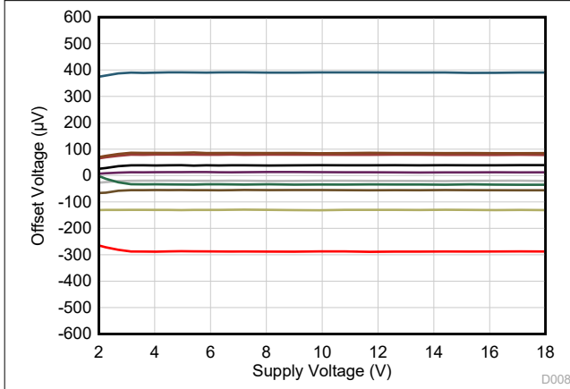
Figure 6-9. Offset Voltage vs Power Supply
