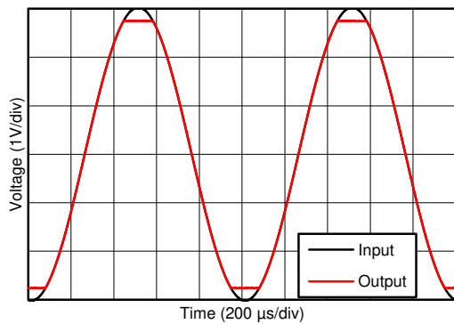
Figure 8-25. No Phase Reversal
