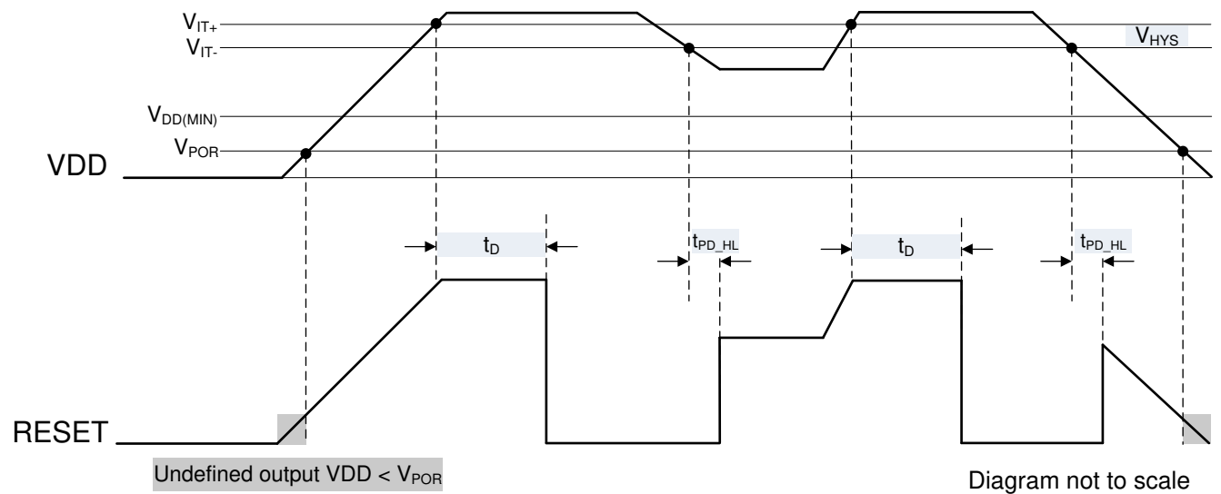
Figure 7-2. TLV810E Timing Diagram
