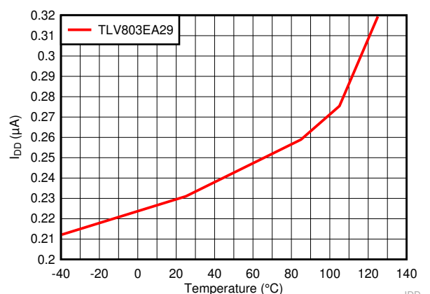
Figure 7-6. Supply Current Versus Temperature for TLV803EA29, V_{DD} = 3.3\text{ V}
