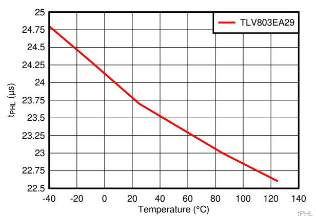
Figure 7-24. High-to-Low Propagation Delay Versus Temperature for TLV803EA29
