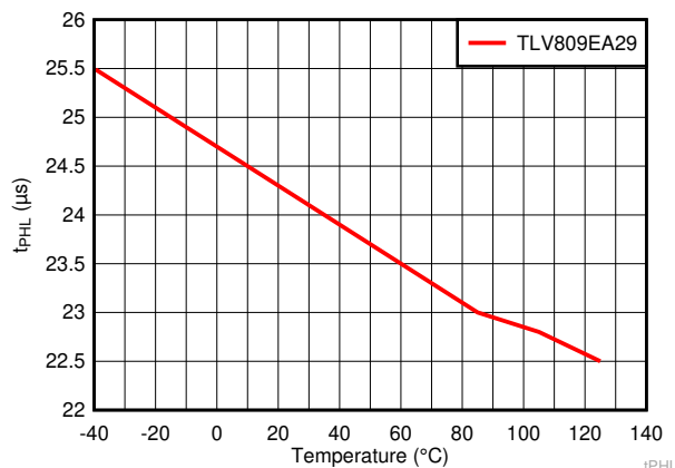
Figure 7-25. High-to-Low Propagation Delay Versus Temperature for TLV809EA29
