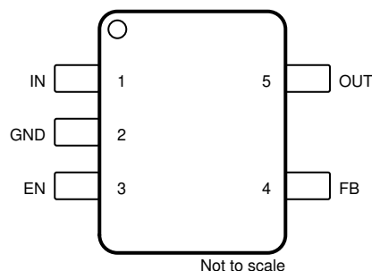
Figure 4-2. DBV Package (Preview), 5-Pin SOT-23 (Top View)
