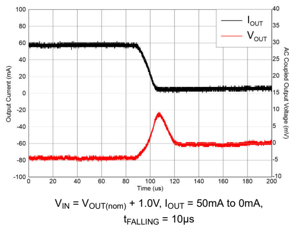
Figure 5-12. Load Transient
