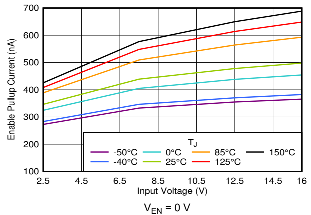
Figure 6-20. I_{EN} vs V_{IN}
