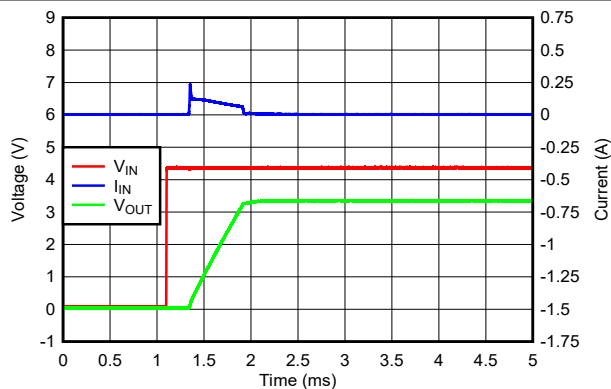
Figure 7-8. Inrush Current With 22\text{ }\mu\text{F} at C_{OUT}
