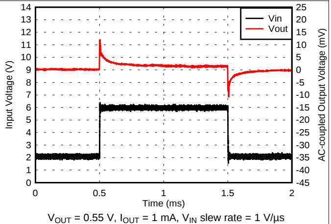
Figure 18. 0.55-V Line Transient
