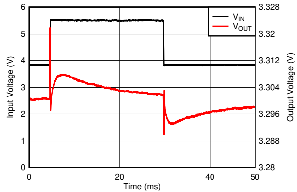
Figure 5-8. Line Transient
