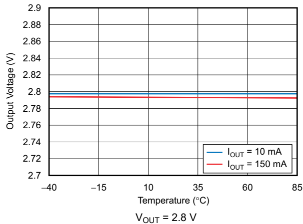
Figure 6-11. Output Voltage vs Temperature
