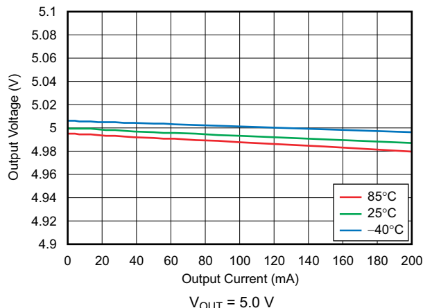
Figure 6-3. Load Regulation
