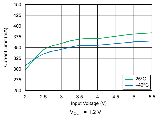
Figure 6-29. Current Limit vs Input Voltage
