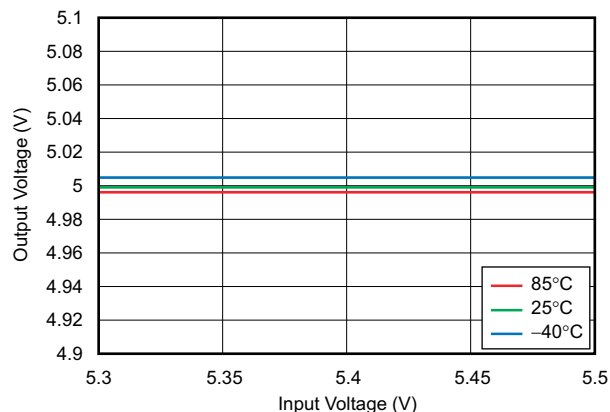
Figure 6-4. Line Regulation
