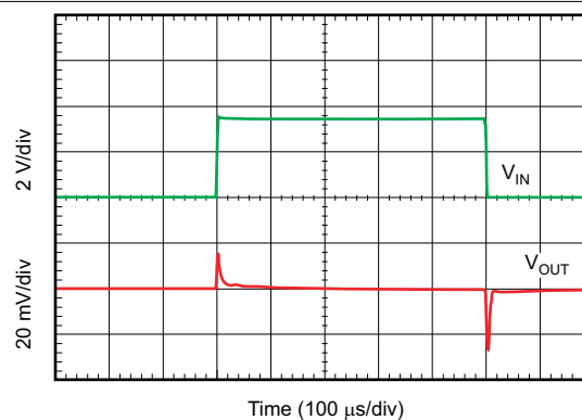
Figure 8-5. Line Transient Response
