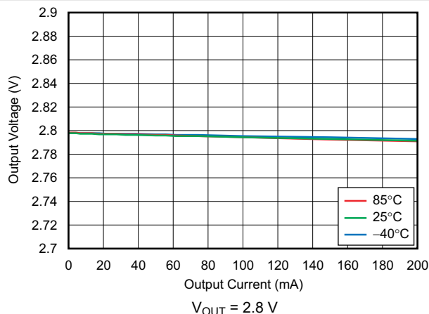
Figure 6-2. Load Regulation
