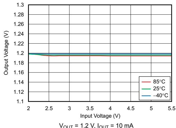
Figure 6-4. Line Regulation
