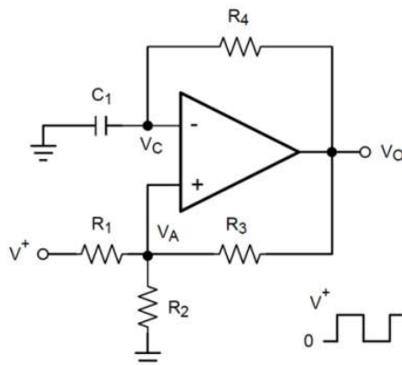
Figure 7-7. Square-Wave Oscillator
