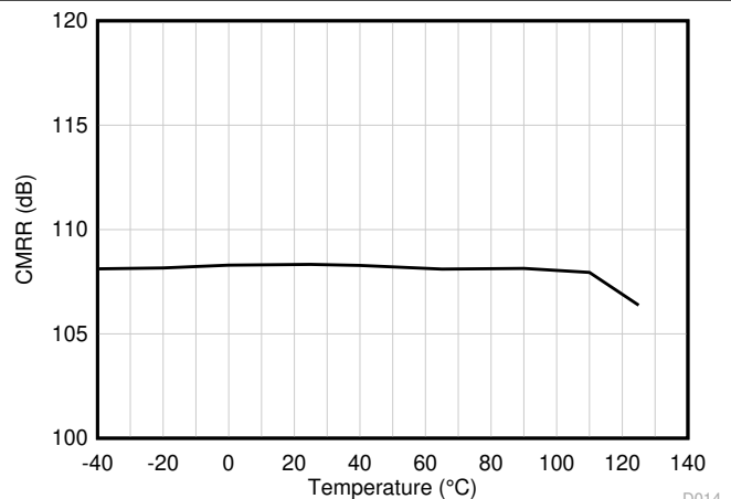
Figure 7-52. CMRR vs Temperature V_S = 5.5\text{ V} , V_{CM} = V_- \text{ to } (V_+) - 1.2\text{ V}
