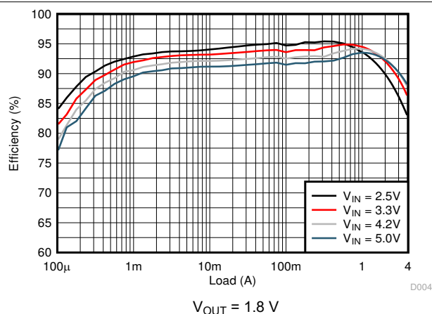
Figure 8-6. Efficiency
