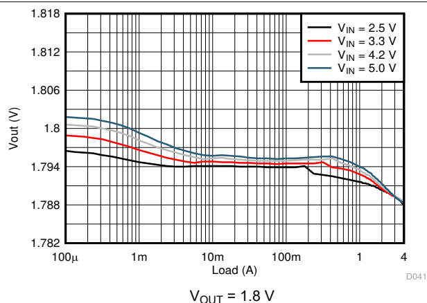
Figure 8-7. Load Regulation
