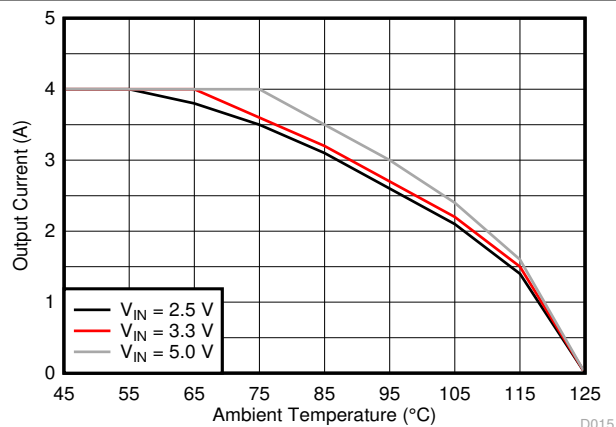
Figure 8-15. Thermal Derating
