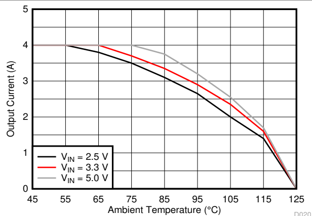
Figure 8-14. Thermal Derating
