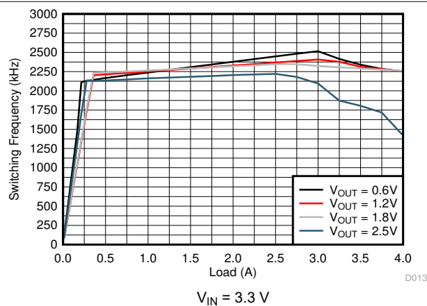
Figure 8-12. Switching Frequency
