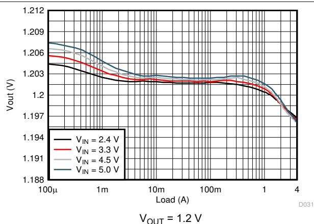
Figure 8-5. Load Regulation
