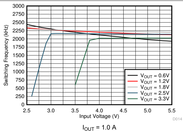
Figure 8-13. Switching Frequency
