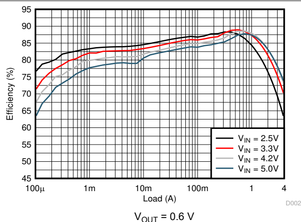
Figure 8-2. Efficiency
