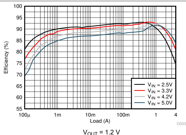
Figure 8-4. Efficiency
