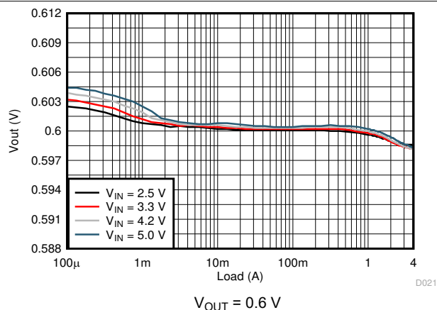
Figure 8-3. Load Regulation
