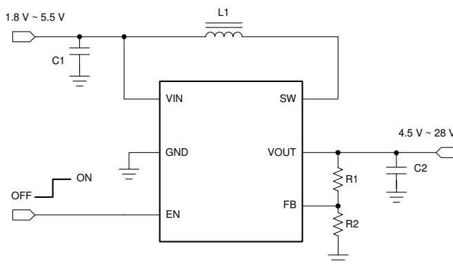
Simplified Schematic
