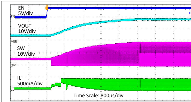
Figure 7-2. Start-up by EN Waveforms
