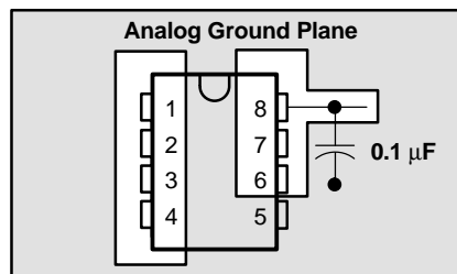
Figure 16. Power-Supply Bypassing
