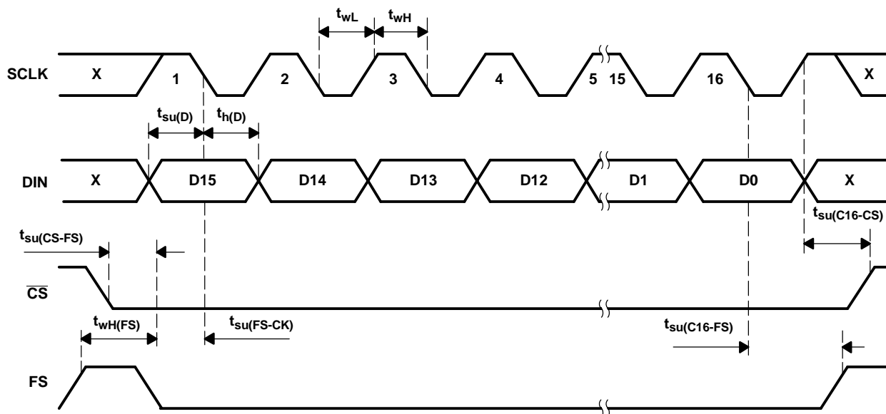
Figure 1. Timing Diagram
