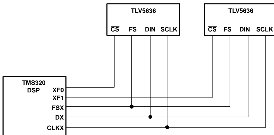
Figure 13. TMS320 Interface
