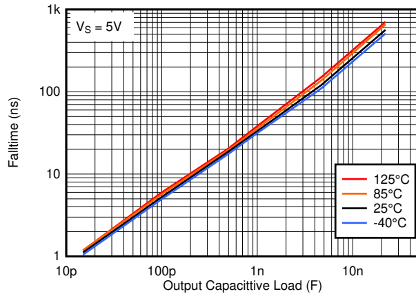
Figure 6-13. Falltime vs. Capacitive Load
