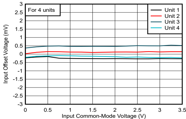
Figure 6-21. Offset Voltage vs. Common-Mode at 25°C, 5V
