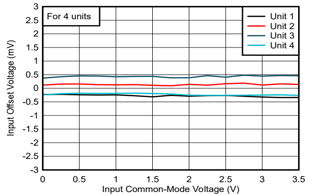
Figure 6-22. Offset Voltage vs. Common-Mode at -40°C, 5V
