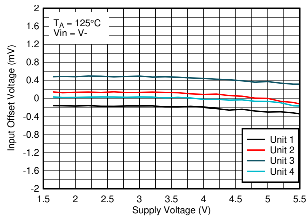
Figure 6-23. Offset Voltage vs. Supply Voltage at 125°C, V_{\text{IN}}=V_-
