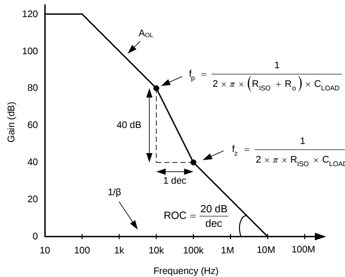
Figure 31. TIPD128 Unity-Gain Amplifier With R_{ISO} Compensation
