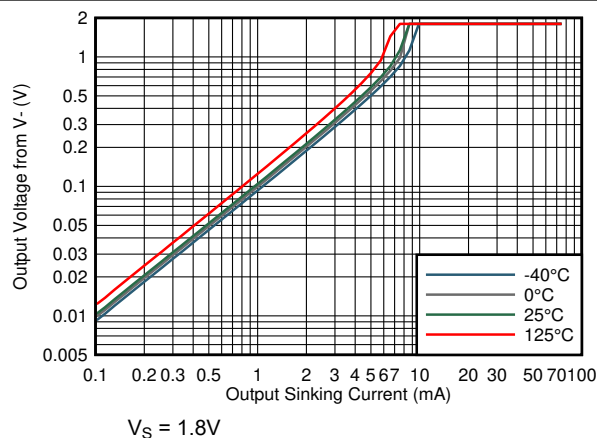
Figure 7-21. Output Voltage vs Output Sinking Current
