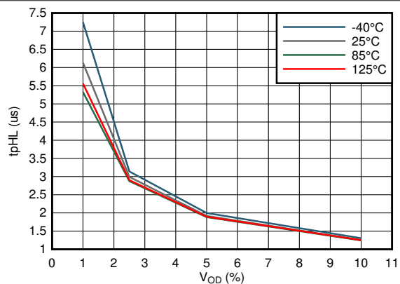
Figure 7-31. Propagation Delay High-Low vs Input Overdrive
