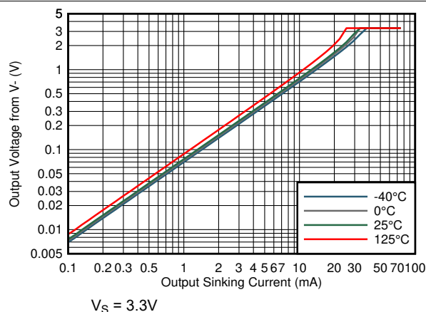
Figure 7-23. Output Voltage vs Output Sinking Current
