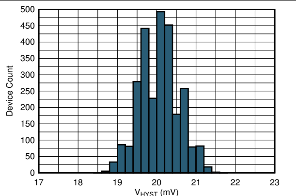
TLV40x1R2 V_S = 5\text{ V} Figure 7-12. Hysteresis Histogram
