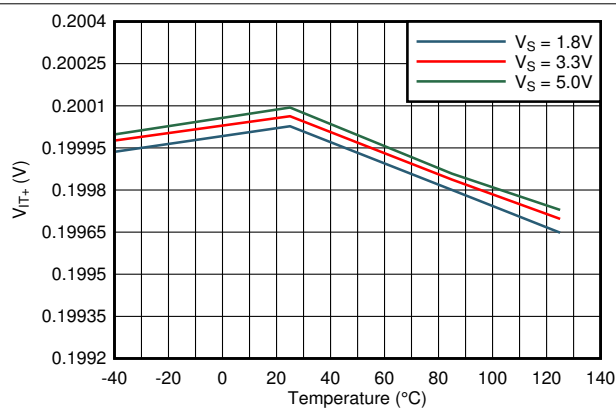
TLV40x1R2 Figure 7-7. Positive Threshold vs Temperature
