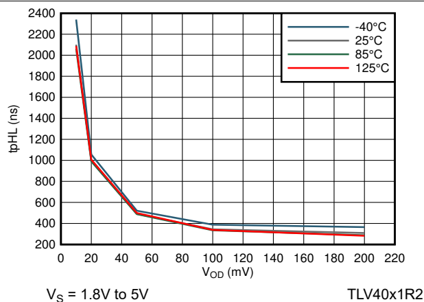
Figure 7-29. Propagation Delay High-Low vs Input Overdrive
