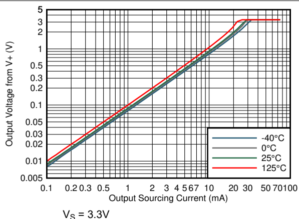
Figure 7-24. Output Voltage vs Output Sourcing Current
