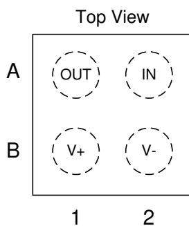
Figure 5-1. YKA Package 4-Bump DSBGA Top View
