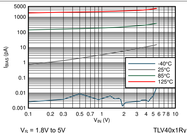
Figure 7-19. Bias Current vs Common Mode Voltage
