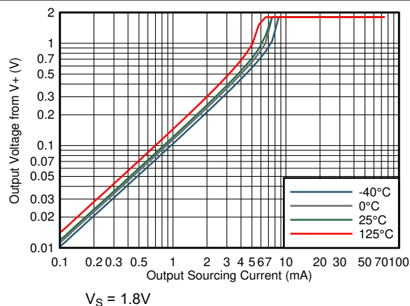
Figure 7-22. Output Voltage vs Output Sourcing Current
