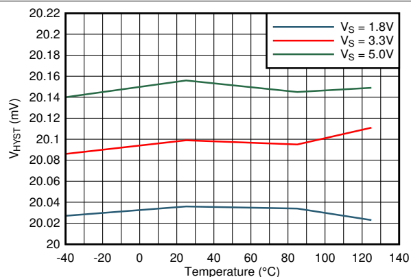
TLV40x1R2 Figure 7-11. Hysteresis vs Temperature
