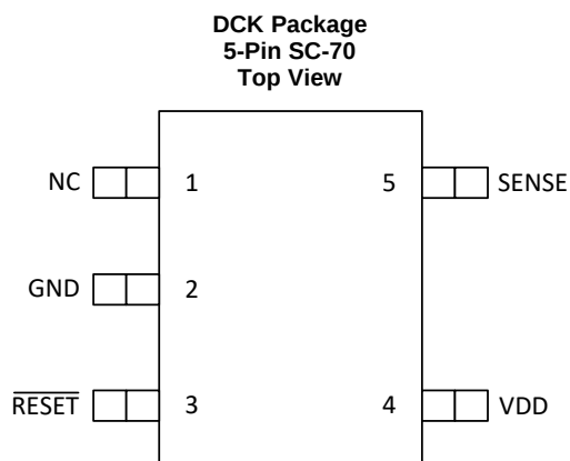
Pin Functions
