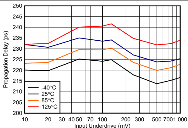
Figure 6-16. Propagation Delay vs. Underdrive, 3.3 V
