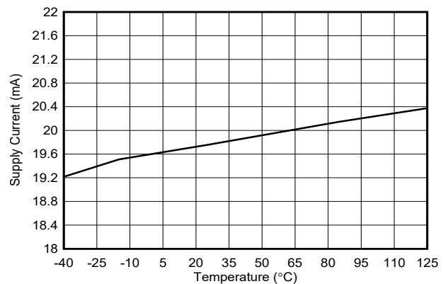
Figure 6-10. Supply Current vs. Temperature, Output High
