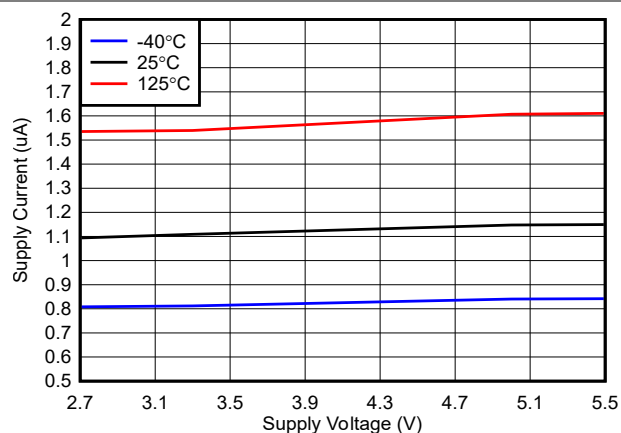
Figure 5-14. Supply Current vs. Supply Voltage (Output High)
