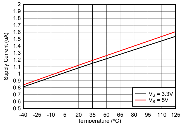
Figure 5-16. Supply Current vs. Temperature (Output High)
