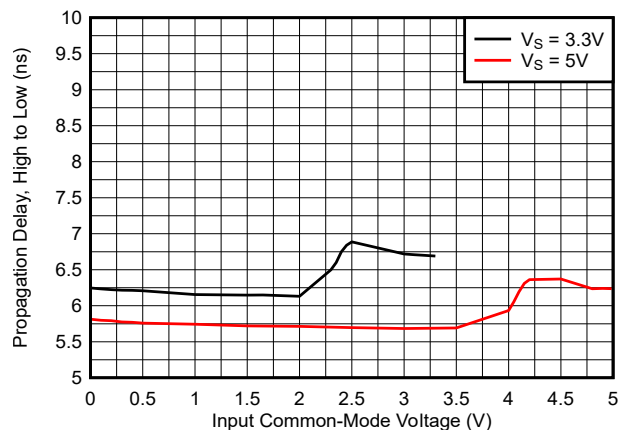
Figure 5-18. Propagation Delay (High to Low) vs. Common-Mode
