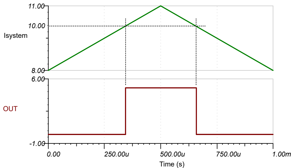
Figure 7-8. Overcurrent Results
