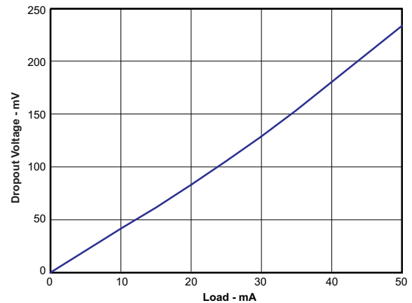
Figure 10. LDO Dropout Voltage vs Load Current
