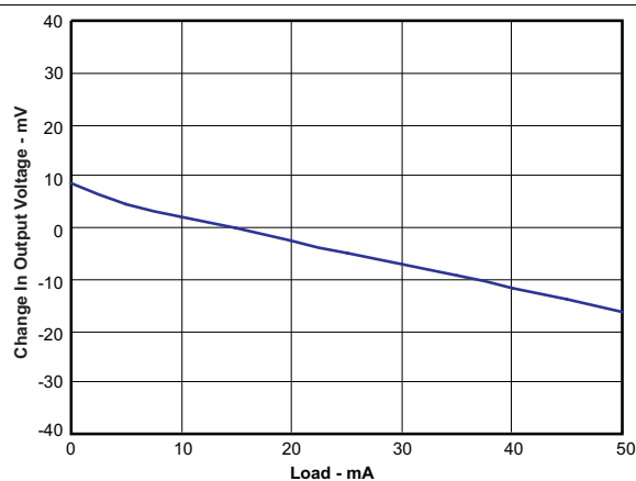
Figure 11. LDO Load Response
