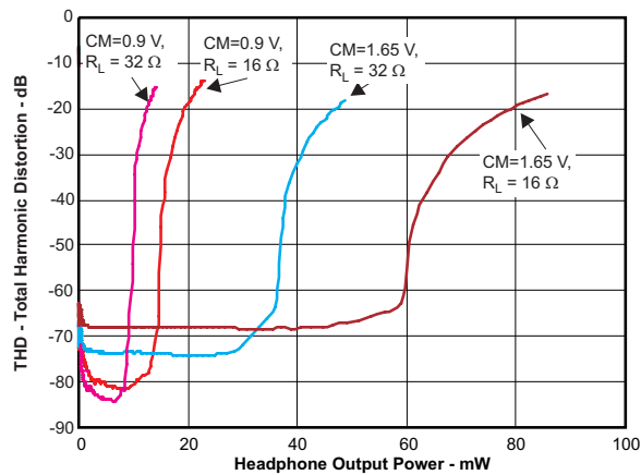
Figure 7. Total Harmonic Distortion vs Headphone Output Power
