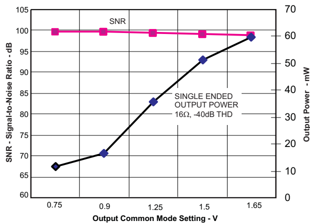
Figure 9. Headphone SNR and SE Output Power vs Output Common Mode Setting
