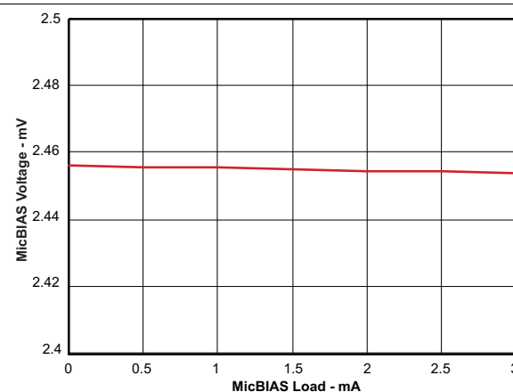
Figure 12. MICBIAS Mode 2, CM = 0.9 V, LDOIN OP Stage vs MICBIAS Load Current
