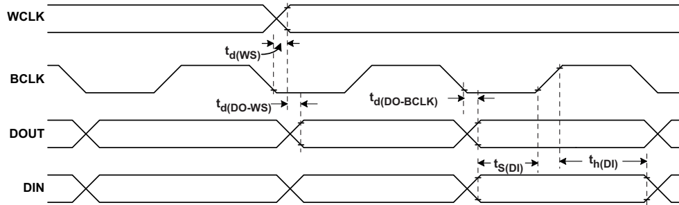
Figure 2. I 2 S, L 2 JF, R 2 JF Timing in Master Mode
