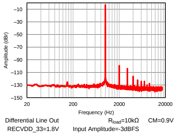
Figure 19. DAC Playback on Line Out Amplifier, Output Amplitude versus Frequency
