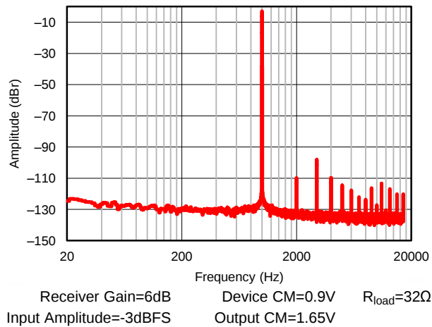
Figure 30. DAC Playback on Receiver Amplifier, Output Amplitude versus Input Frequency
