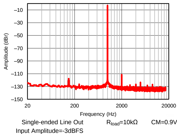
Figure 22. DAC Playback on Line Out Amplifier, Output Amplitude versus Frequency
