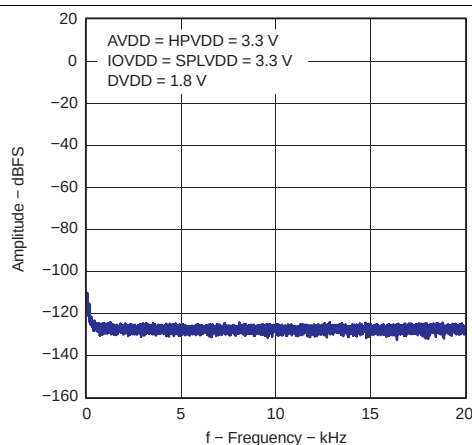
Figure 5-9. FFT – ADC Idle Channel, Single-Ended
