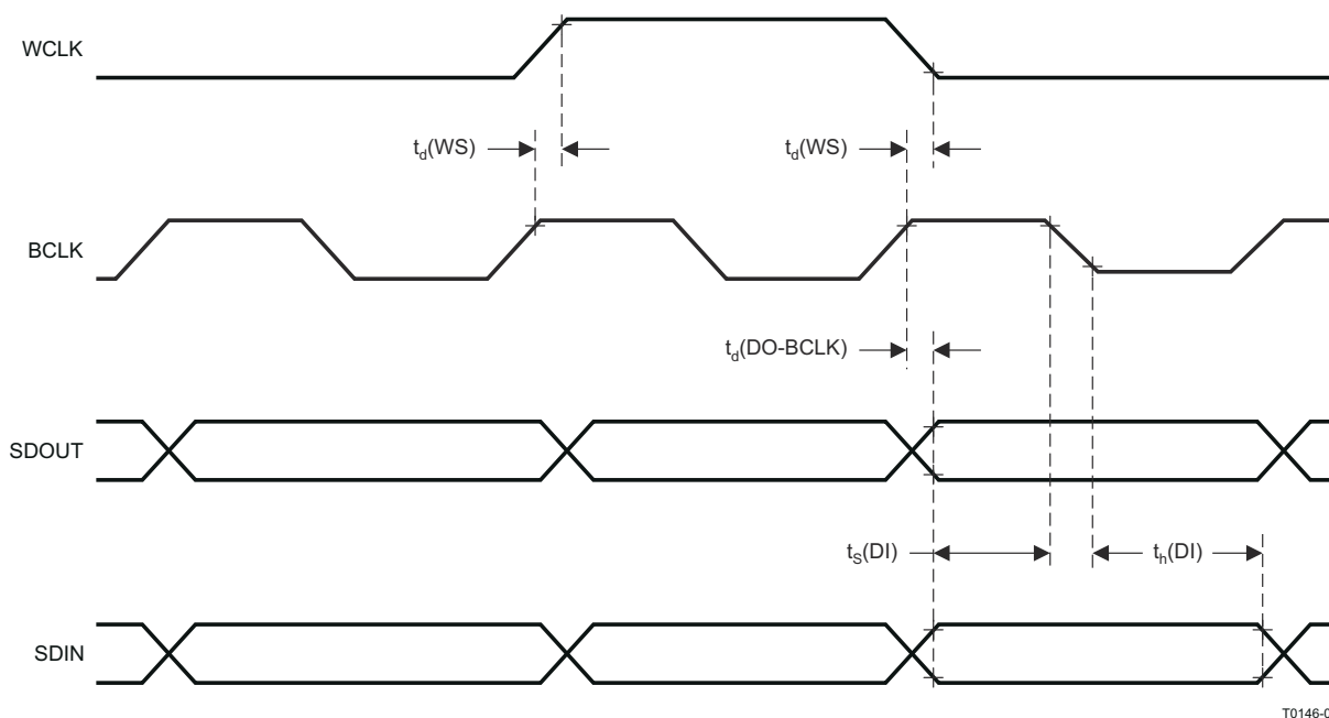
Figure 8-2. DSP Timing in Master Mode
