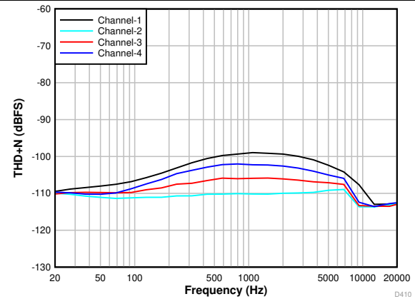
Figure 12. THD+N vs Input Frequency With a -1-dBr Input
