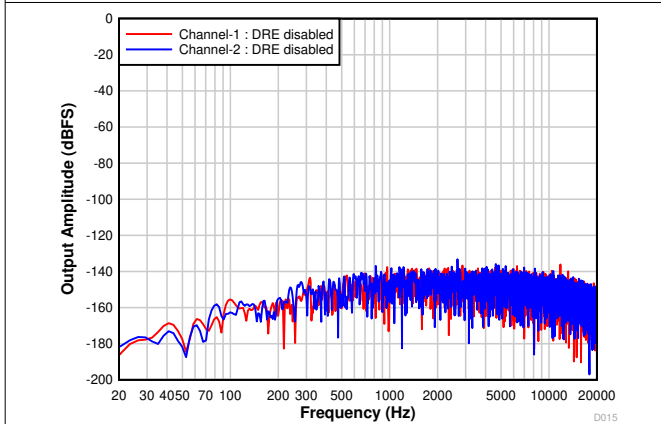
Figure 7-18. FFT With Idle Input With DRE Disabled
