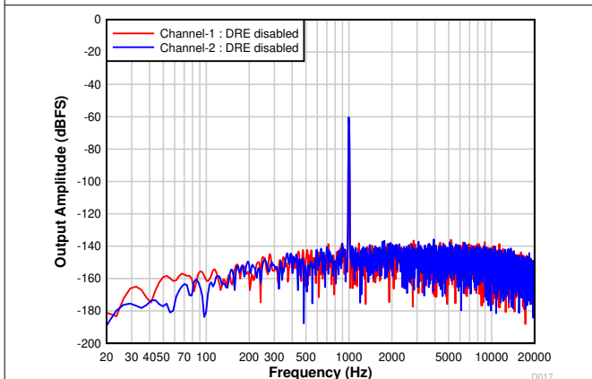
Figure 7-20. FFT With a -60-dB Input With DRE Disabled
