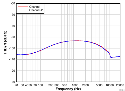
Differential input with high CMRR mode
