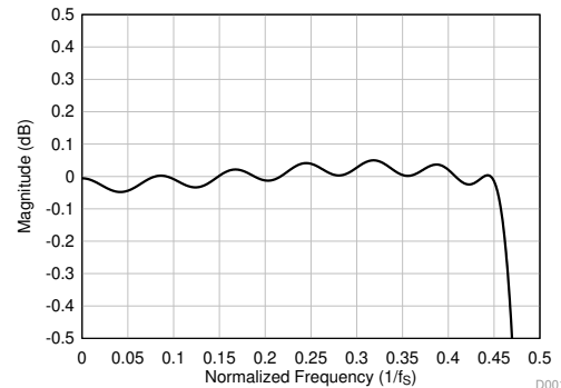
Figure 38. Linear Phase Decimation Filter Pass-Band Ripple
