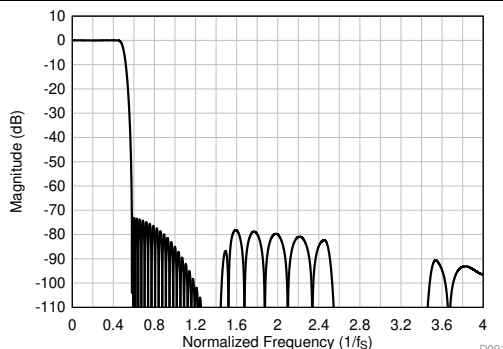
Figure 39. Linear Phase Decimation Filter Magnitude Response
