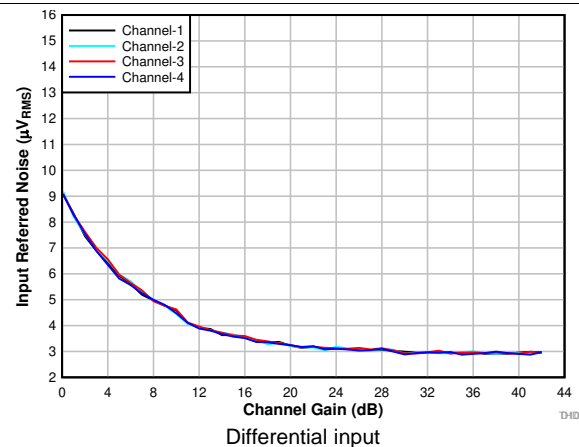
Figure 10. Input-Referred Noise vs Channel Gain
