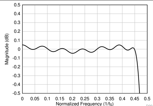
Figure 40. Linear Phase Decimation Filter Pass-Band Ripple
