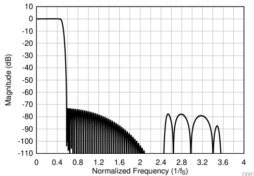
Figure 37. Linear Phase Decimation Filter Magnitude Response
