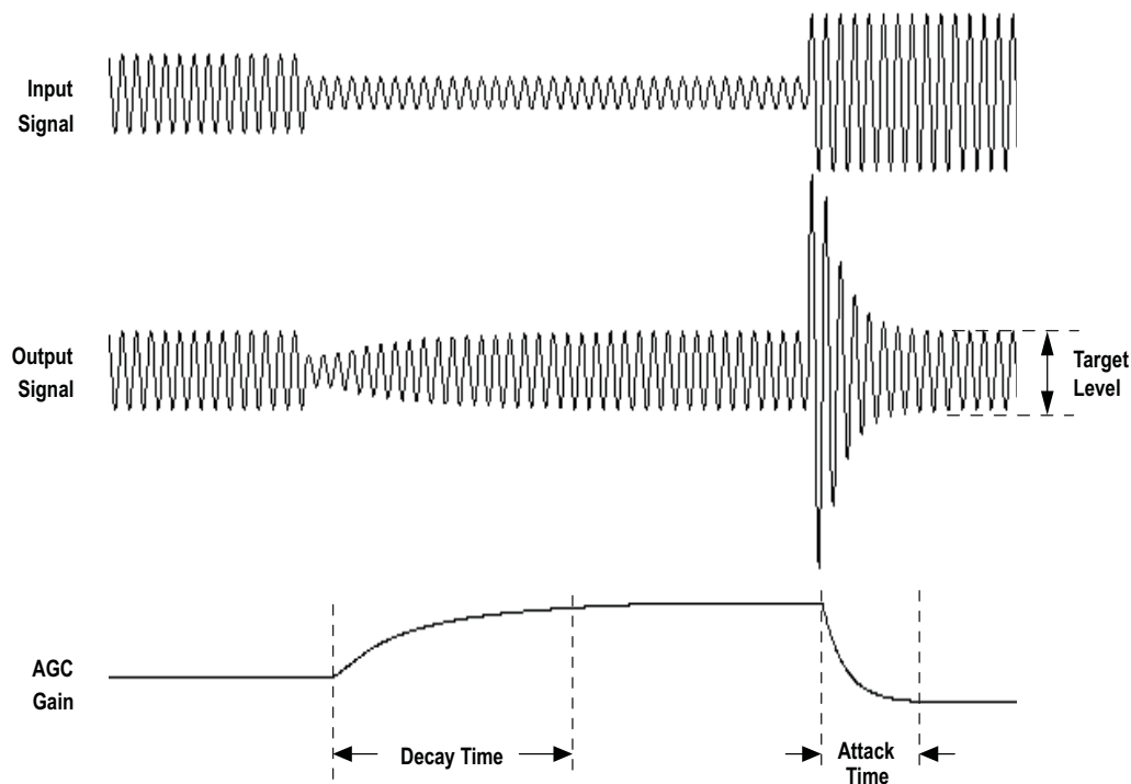
Figure 28. AGC Characteristics
