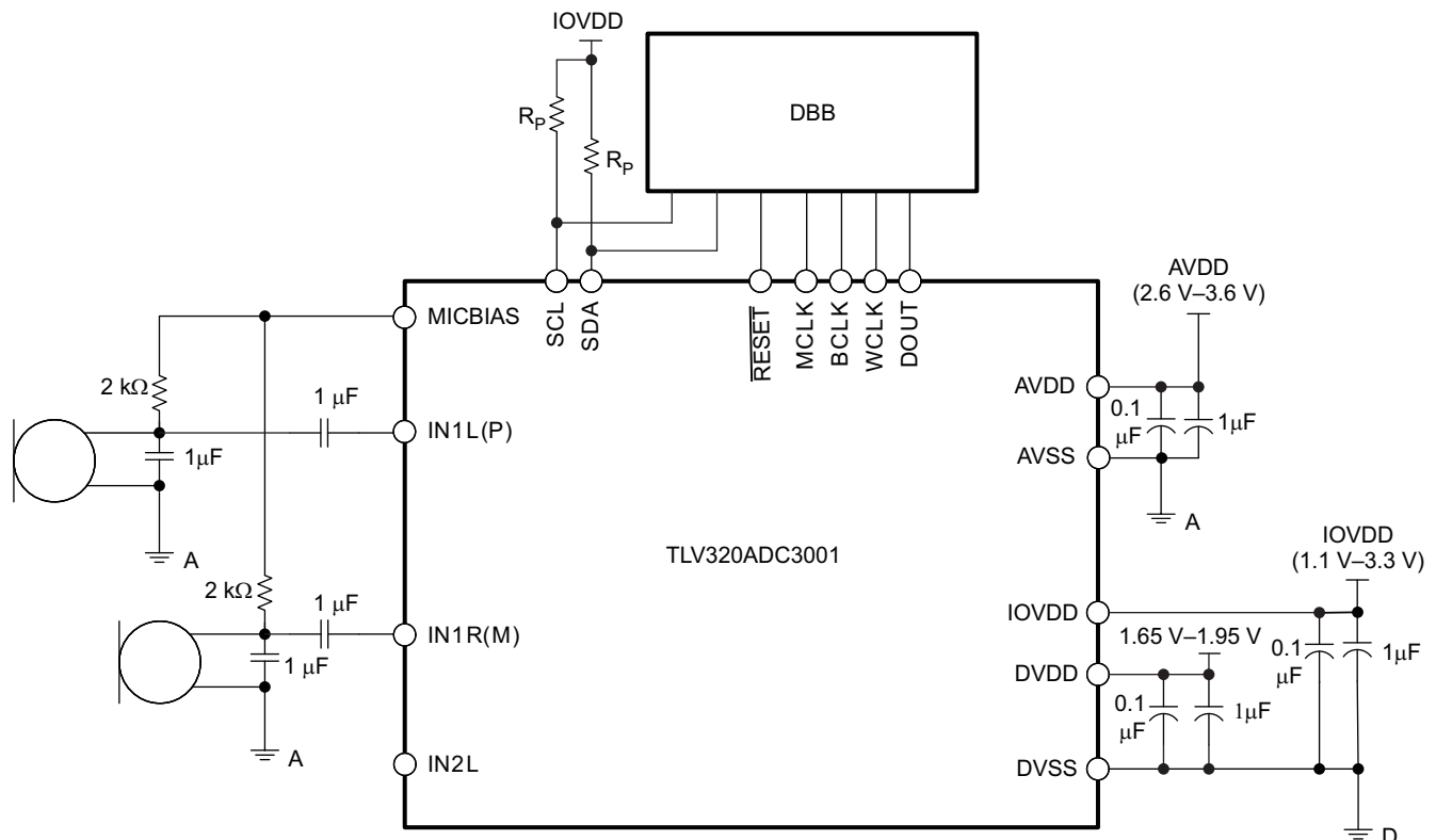
Figure 44. Typical Connections
