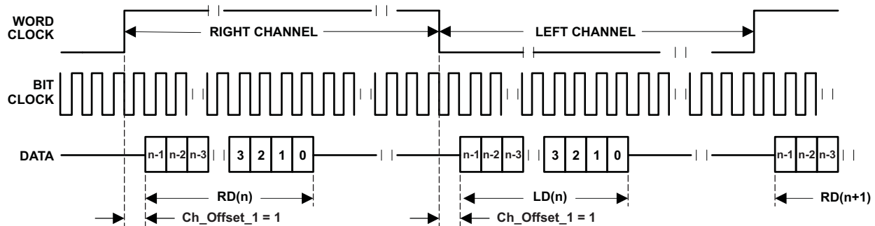
Figure 16. Left-Justified Mode With \text{Ch\_Offset\_1} = 1 , Channel Swapping Enabled
