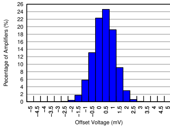
Figure 6-1. Offset Voltage Distribution
