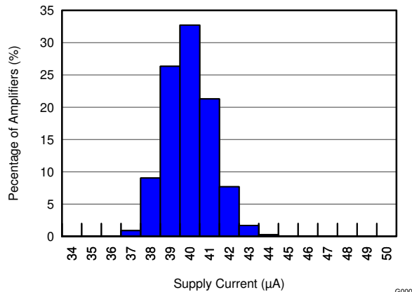
Figure 6-11. Quiescent Current Distribution
