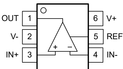
Figure 4-1. DCK, DBV Package 6-Pin SC-70, SOT-23 Top View
