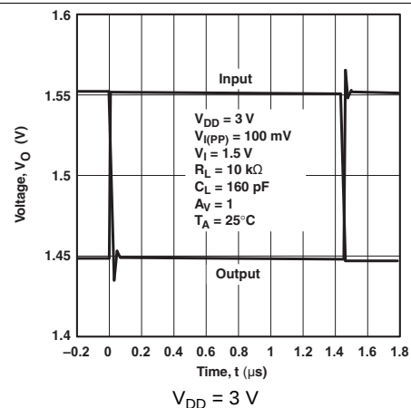
Figure 46. Inverting Small Signal
