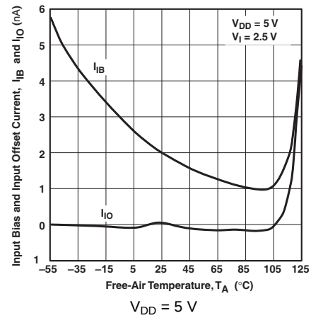
Figure 4. Input Bias and Input Offset Current vs Free-Air Temperature
