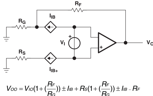
Figure 50. Output Offset Voltage Model
