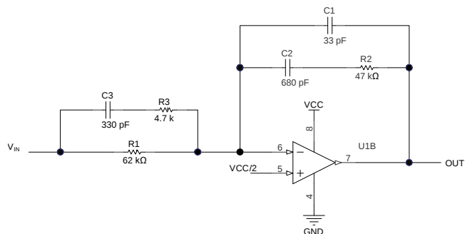
Typical Application
