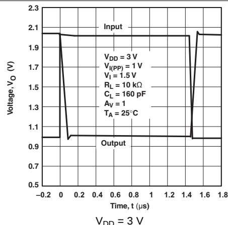
Figure 44. Inverting Large Signal
